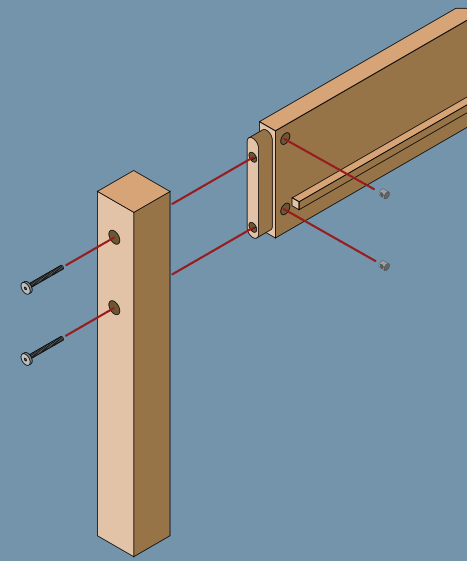
Sturdy mortise & tenon joints each secured with two bolts and barrel nuts
