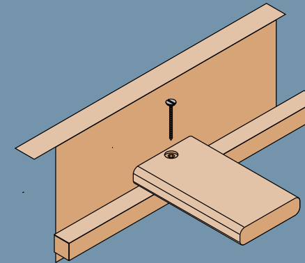
Both 14 piece slat kits secure to bed rails to prevent collapse and add extra stability
